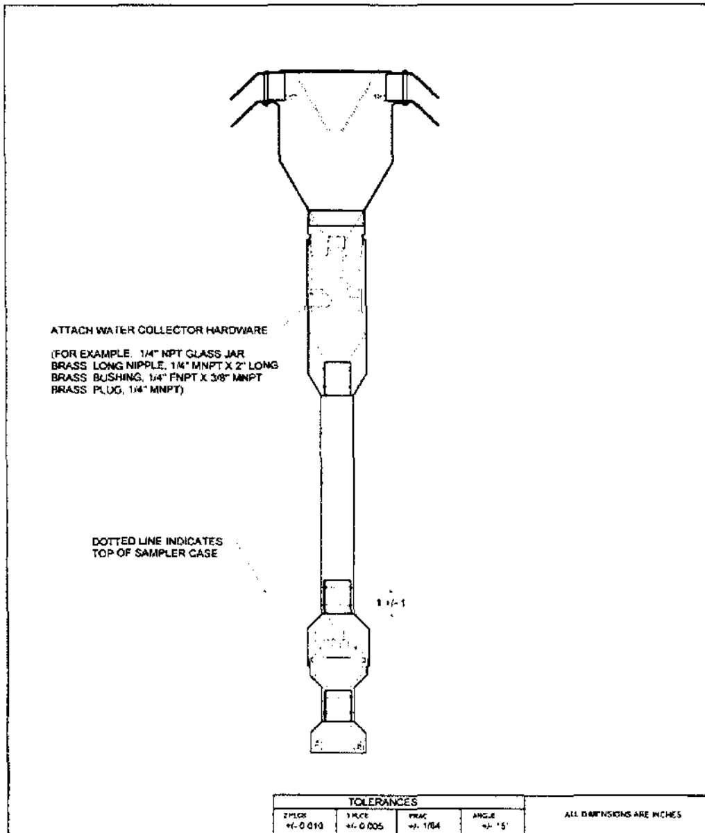
FIGURE L-1. PM2.5 SAMPLER, ASSEMBLY
