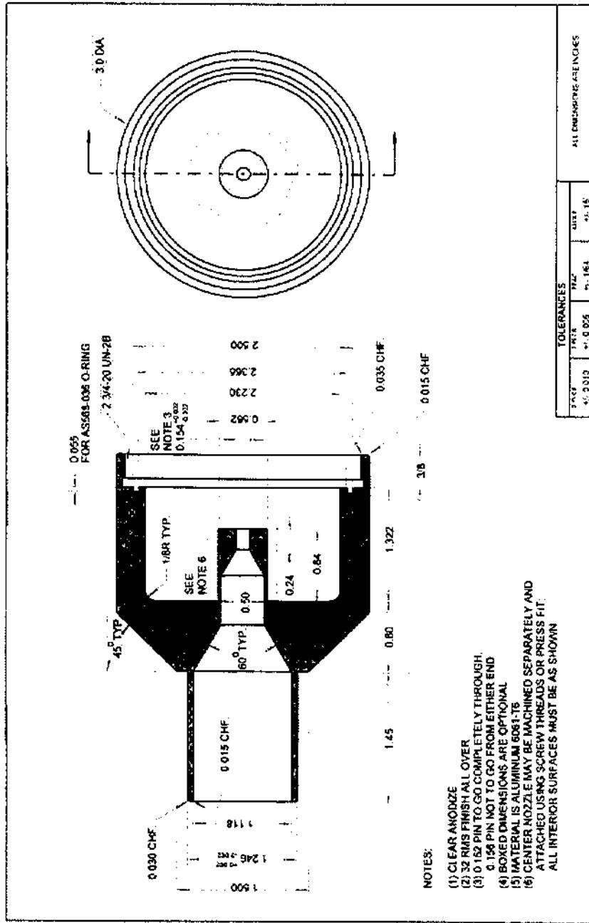
FIGURE L-21. 2.5-MICRON IMPACTOR HOUSING, UPPER
