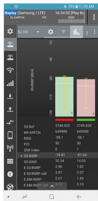
Fig. 15: PCI and SSB based real-time EMF measurement values in mV/m
