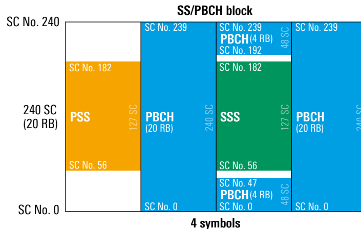
Fig. 4: 5G NR synchronization signal block
