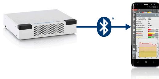
Fig. 12: R&S®TSMA6 and Android smartphone connected via Bluetooth®
