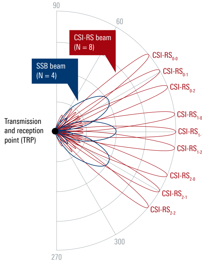
Fig. 9: UE specific signal component (CSI-RS) is transmitted using extremely narrow beams compared to SSB beams
