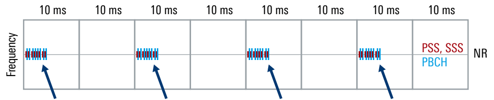
Fig. 6: Periodically broadcasted synchronization signal blocks
