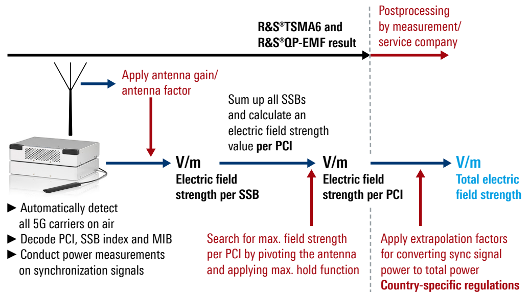
Fig. 11: Typical EMF measurement procedure for code-selective maximum emission measurements in 5G NR
