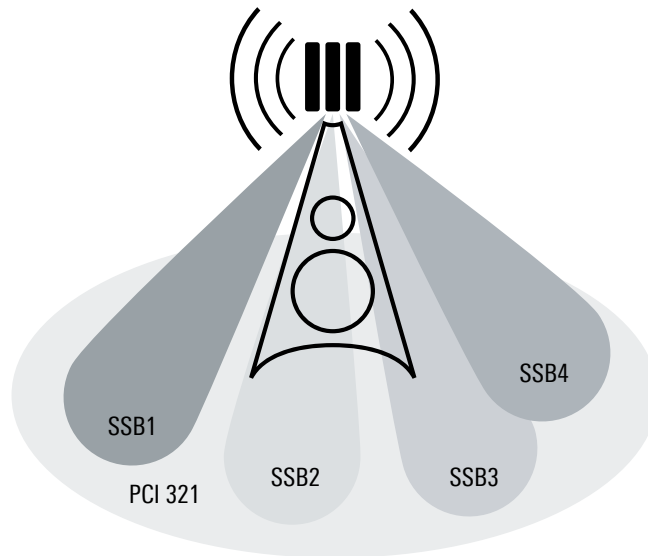
Fig. 1: 5G NR cell with PCI 321 is divided into several synchronization beam areas (SSB)
