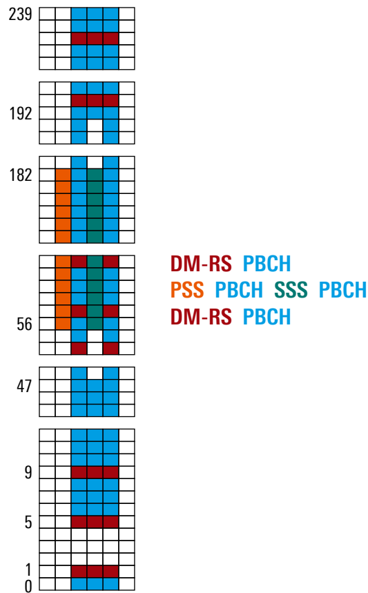
Fig. 5: 5G NR synchronization signal block with increased zoom factor
