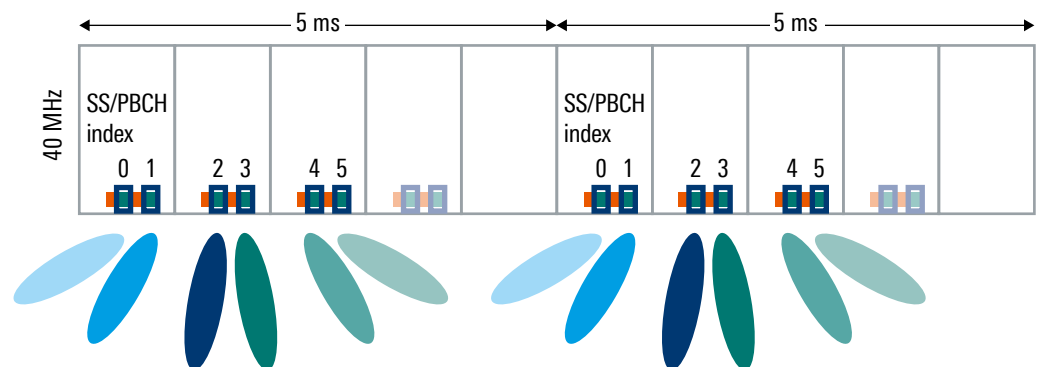
Fig. 7: Example of SSB transmissions
