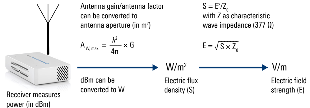
Fig. 3: Relationship of power, electric flux density (S) and electric field strength (E)
