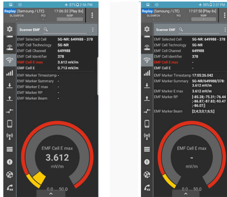
Fig. 14: QualiPoc screenshots when searching for the max. electric field strength in mV/m (left) and marking the cell after the maximum is found (right)
