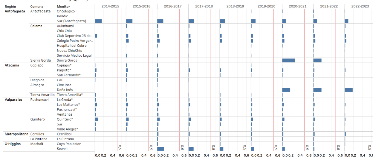
Promedio bianual de Pb ( \mu\text{g}/\text{m}^3 )
