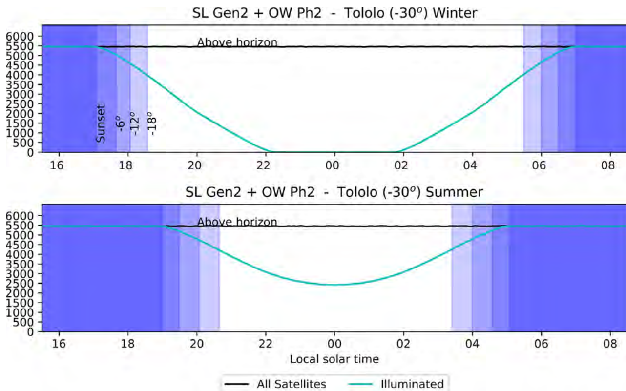
Figure 6.1.1. Evolution over the night of the number of satellites above the horizon at latitude 30^{\circ} south (representative of Cerro Tololo and Cerro Pachón, for instance) on winter and summer solstices. The black curves show the total number of satellites above the horizon (illuminated or not), while the cyan curve shows only those that are detectable, because they are illuminated by direct sunlight. Sunset, sunrise and the various twilights are indicated with shading: the white area corresponds to astronomical night. While in winter the number of detectable satellites plummets towards the middle of the night, in summer many satellites remain illuminated and above the horizon even at midnight. O. Hainaut.
