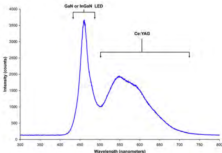
Figure 3.6: Spectral energy distribution of a typical high-correlated colour temperature (CCT) white LED with a strong peak in the blue at wavelength about 465 nm. Wavelength ranges above the SPD indicate the colors for which the LED semiconductor material (GaN and InGaN) or phosphor coating (Ce:YAG) are responsible. (Courtesy of Deglr6328; This image is licensed under the Creative Commons Attribution-Share Alike 3.0 Unported license. Original source on Wikipedia https://en.wikipedia.org/wiki/Light-emitting_diode )
