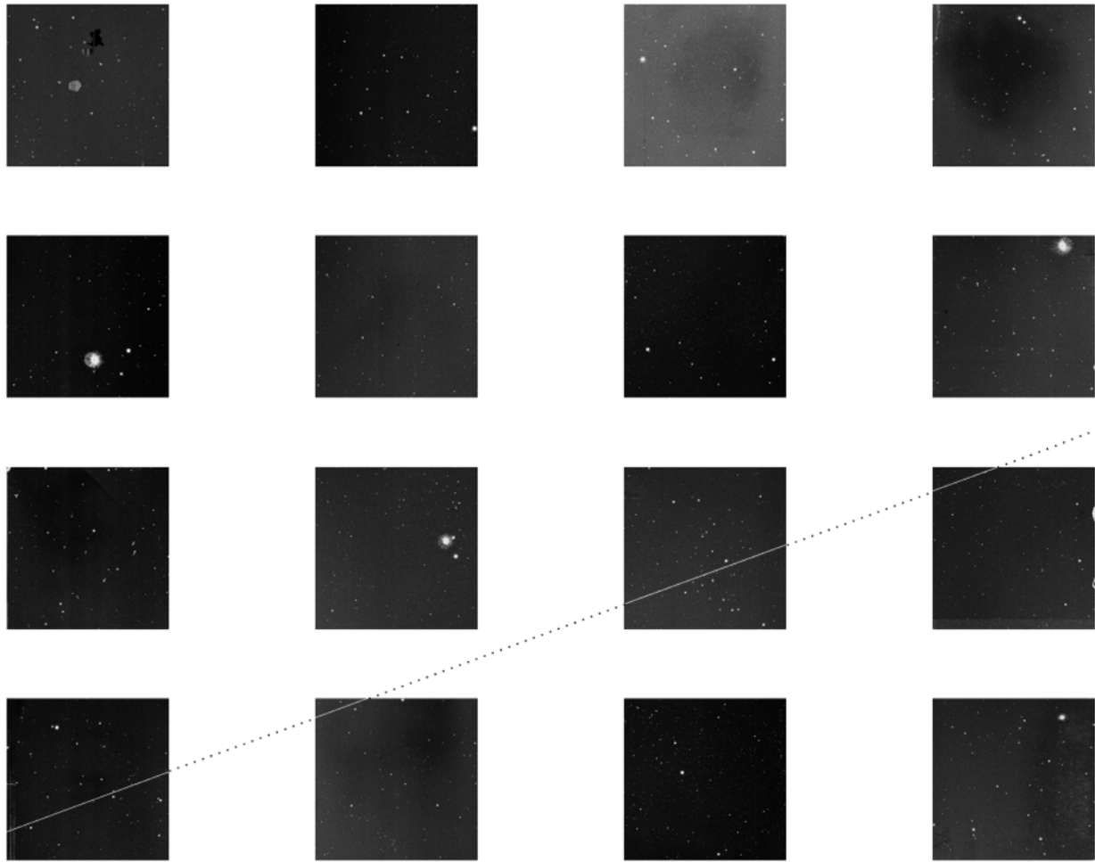
Figure D.2.12 NIR image of DarkSat taken using a J filter with VIRCcam on the 4m VISTA telescope, ESO Cerro Paranal Observatory, Chile. The 16 CCD images (11.6 x 11.6 arcmins) are arranged in geometric order and the gaps between the detectors are to scale. With the horizontal and vertical gaps between the detectors corresponding to 10.4 arcmins and 4.9 arcmins, respectively. The dotted line represents the satellite trail falling within the detector gaps.
