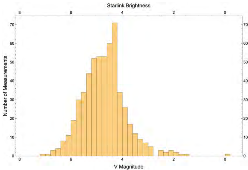
Figure D.2.15. A histogram of 567 Johnson V magnitude measurements of Starlink satellites imaged by the POMENIS Observatory from May to September 2020. The mean of all 567 measurements is 4.7 with a standard deviation of 0.85. This broad distribution of values demonstrates the varied brightness of Starlink satellites which depends on numerous geometric factors. Note there are additional observations of Starlink satellites that are fainter than 6th magnitude for which the SNR is too low to be processed by the current software pipeline.
