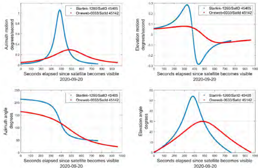
Figure D.2.3. Azimuth, elevation angular motion (top plots) and azimuth and elevation position above the horizon (bottom plots) for satellites Starlink-1260 (550 km orbital height at the time of the observation) and OneWeb-0033 (960 km orbital height at the time of the observation), as seen from the location of the Ckoirama Observatory in northern Chile.
