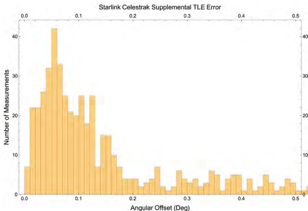
Figure D.2.5. The majority of TLE predictions are less than 0.2 degrees off from the actual satellite position. Large errors are present and extend all the way to >0.5 degrees, the limit of the telescope's FOV and thus ability to measure.
