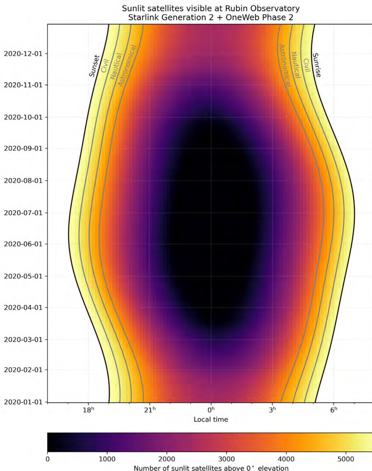
Figure 6.1.4. Bulk number of satellites of the constellation SL2+OW2 that are above horizon and illuminated from latitude 30° south (Cerro Pachón, Cerro Tololo) as a function of both local time (horizontal axis) and date of the year (vertical axis). The white area corresponds to daytime (Sun above horizon). Curved lines indicate sunset and sunrise, and the times of the different twilights. Compare to the following figure to check the influence of the elevation above the horizon. Colour code runs from zero (black) to more than 5000 (yellow). Figure by C. Bassa using analytic methods.
