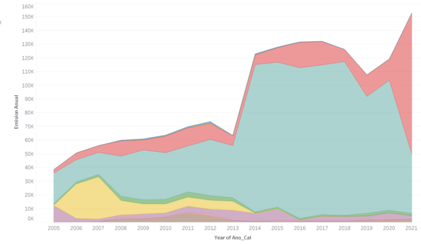
The plot of sum of Emission for Ano_Cal Year. Color shows details about Sector (Clasificación Sectores (Clasificación_Puntuales)). The data is filtered on Ano_Cal Year, Contaminante and ContaminantesNCAire. The Ano_Cal Year filter excludes 2022. The Contaminante filter keeps CO. The ContaminantesNCAire filter keeps 4 members.
